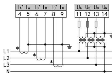
3P 4W, 3CT, 3PT
