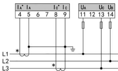
3P 3W, 2CT, без PT
